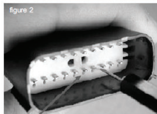
Wiring Worksheet - LEFT (Grey)
