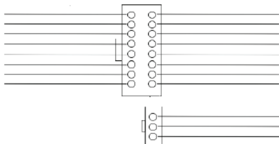
Wiring Worksheet - RIGHT (Black)
